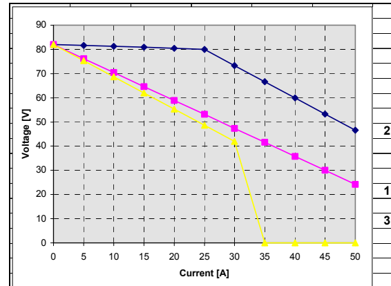
Figure 13. Current-voltage characteristic of different power supply topologies.
