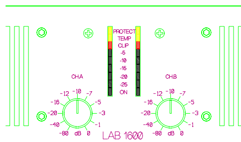
Figure 12. Front indicators
