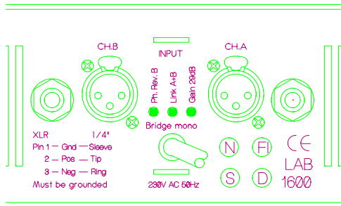
Figure 5. Rear panel connectors
