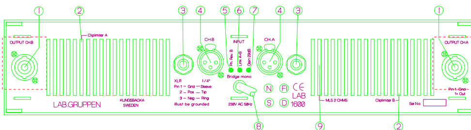
Figure 2. Rear panel
