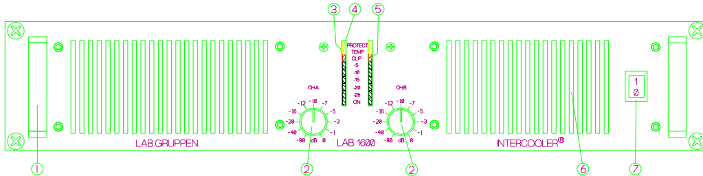
Figure 1. Front panel
