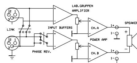
Figure 10. Bridge mono connection
