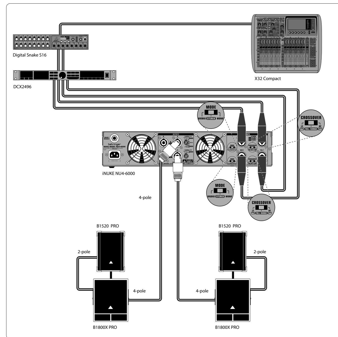
Vertical Bi-amping/Bi-amplificación vertical/Bi-amplification verticale/Vertikales Bi-Amping/Bi-amplificação Vertical
