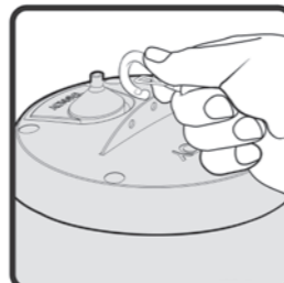
6. Attach the hanging cable to the centre hole of the speaker bracket. The safety cable can be attached to either of the secondary holes.
