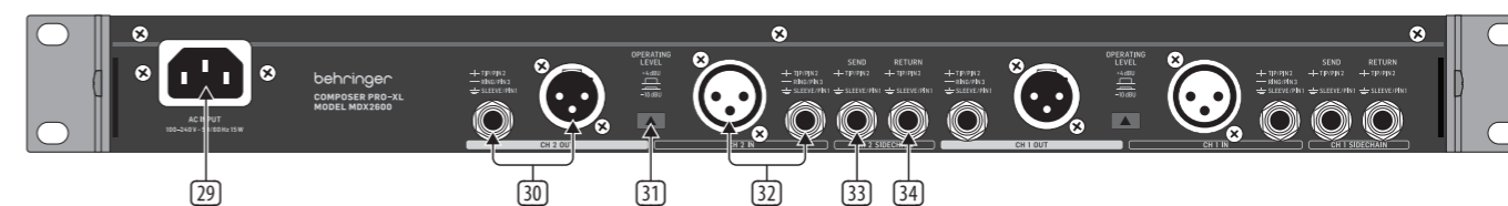
MDX2600 rear panel
