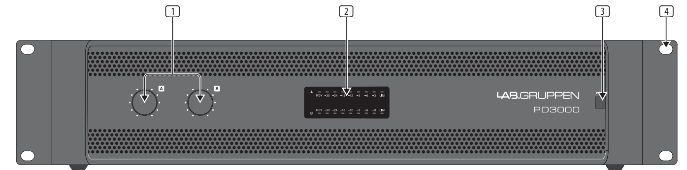
Fig. 1: Painel frontal do PD3000
