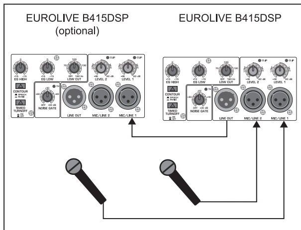
Fig. 4.1: Connecting microphones
