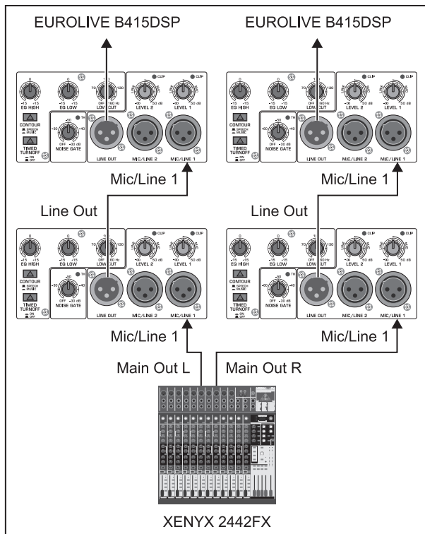
Fig. 4.3: Linking several B415DSP speakers
